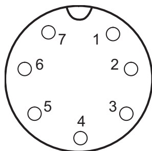
Figure 11.2: Power supply plug, 7-pole (rear view of plug, solder side)
