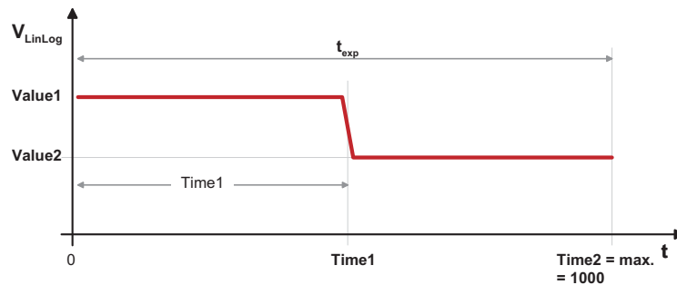
Figure 4.11: Voltage switching in the Linlog2 mode
