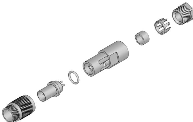
Figure 11.1: Power connector assembly
