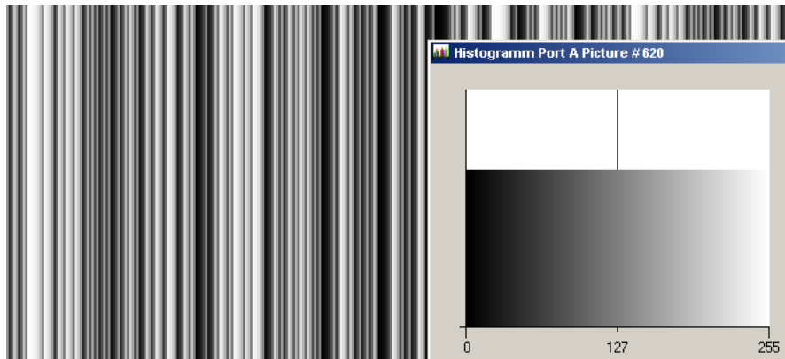
Figure 4.23: LFSR test pattern received at the frame grabber and typical histogram for error-free data transmission
